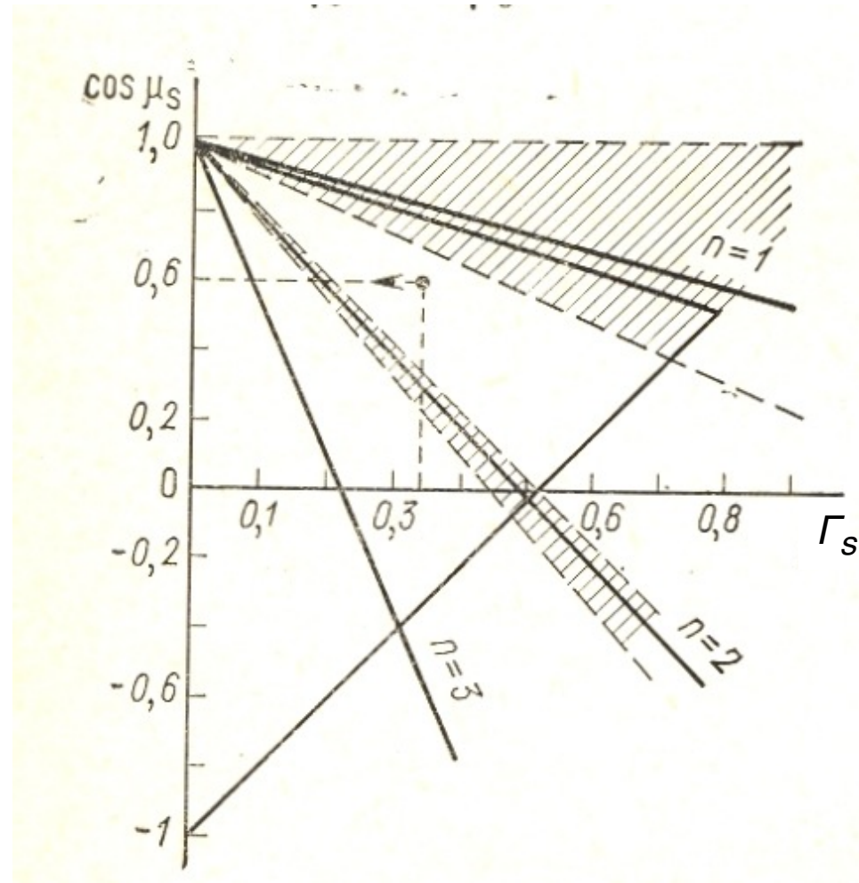
Parametric resonance regions.
