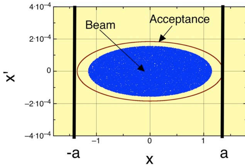
Focusing Quadrupole
