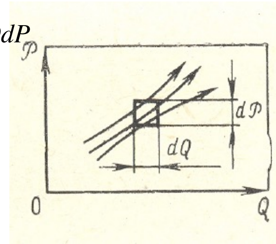
On derivation of Liouville theorem.
