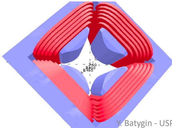
Electromagnetic quadrupole magnet in Maier-Leibnitz Laboratory, Munich
