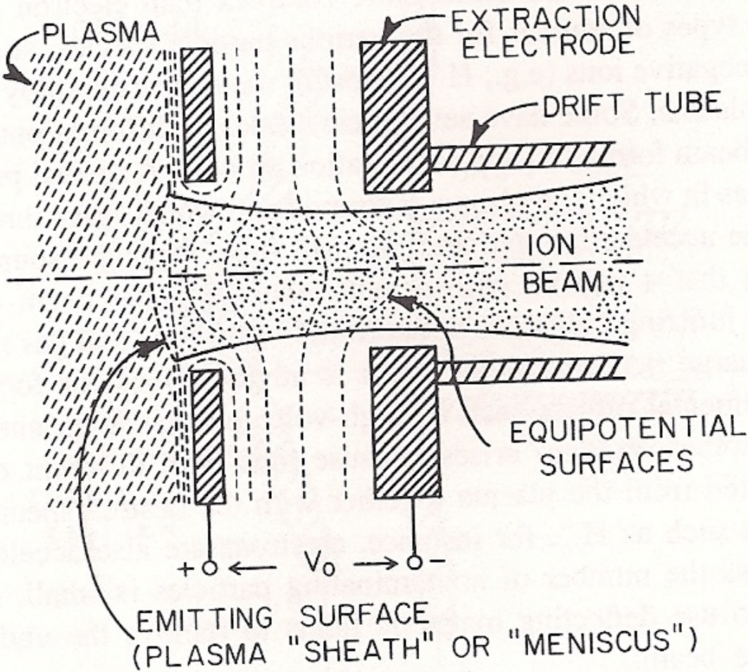
Schematics of a plasma ion source (from M.Reiser, 1994).
