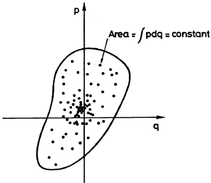
Illustration of conservation of phase space volume
