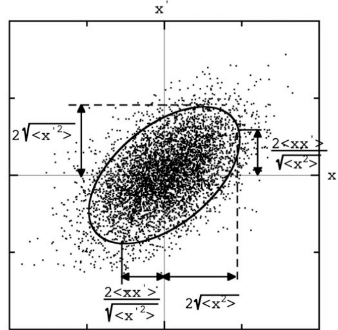
Beam distribution and 4-rms ellipse.
