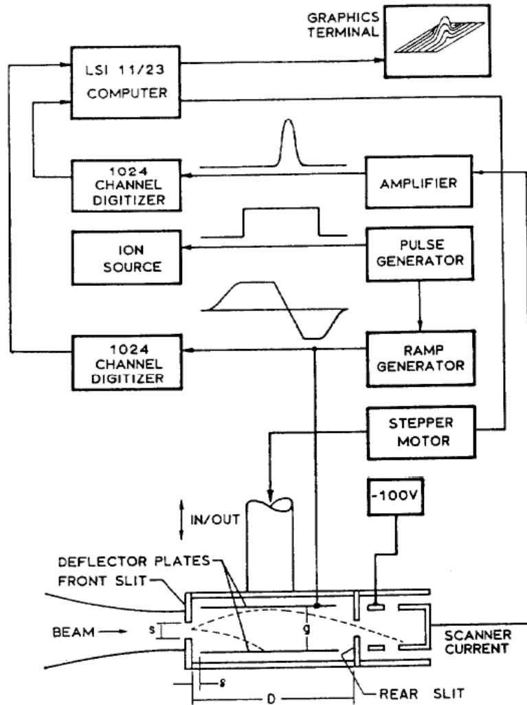
Fig. 1. Schematic of electric-sweep emittance scanner.
