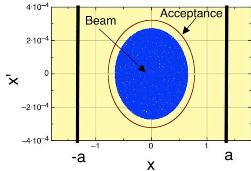
Defocusing Quadrupole
