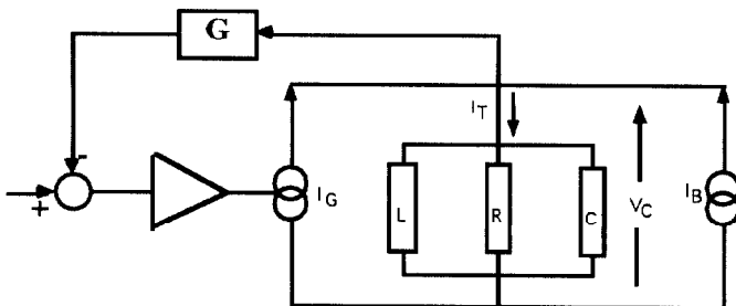
Fig. 1. Simple resonant cavity model driven by a generator and a beam current. RF feedback appears as a transform G of the cavity voltage summed with the klystron drive signal.
