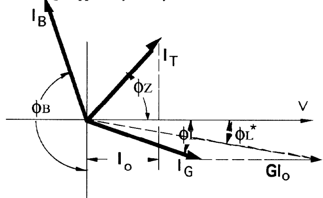
Fig. 2. The current from the generator, the beam and the total current are represented as phasors, referenced to the cavity voltage. The feedback contributes a term G I_0 .
