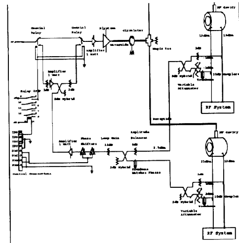
Fig. 5 Schematic of the direct RF feedback implemented around the klystron and two damping ring cavities.
