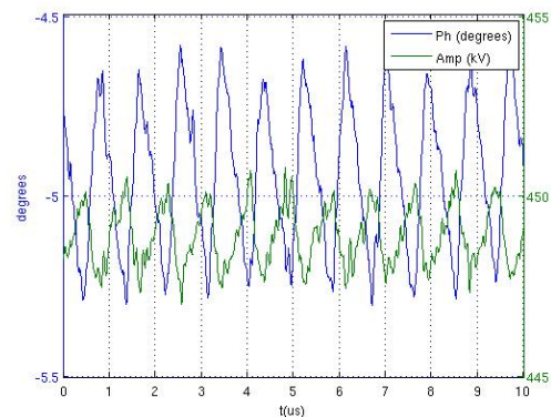
Figure 5: Cavity Voltage and Phase variations per turn due to Beam Loading.
