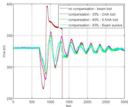
Figure 4: Comparison of different Feed-Forward Settings after a forced RF trip.
