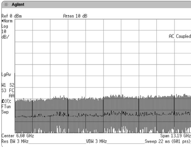
Figure 2-23a. Normal mode
