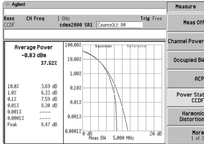
Figure 8-1. CCDF measurement
