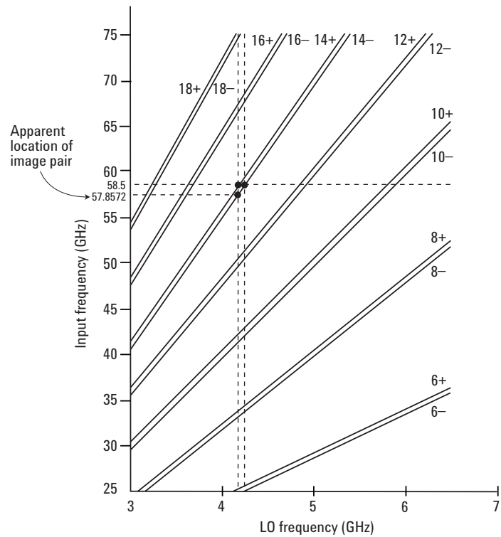
Figure 7-16. Harmonic tuning lines for the E4407B ESA-E spectrum analyzer
