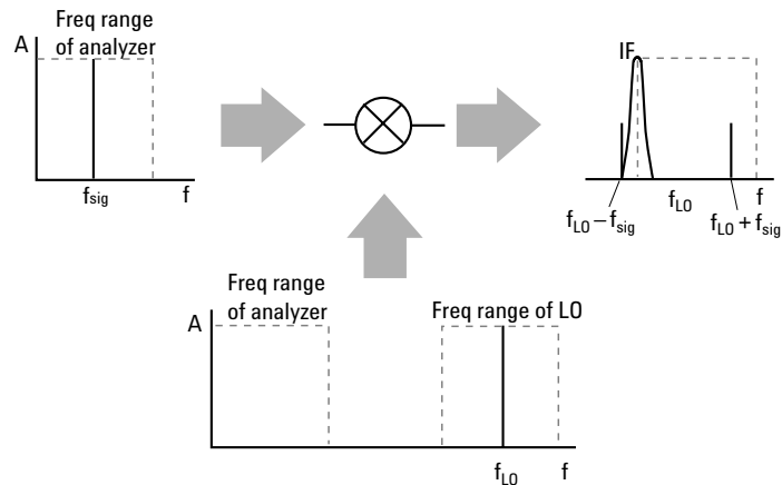
Figure 2-4. The LO must be tuned to f_{IF} + f_{sig} to produce a response on the display
